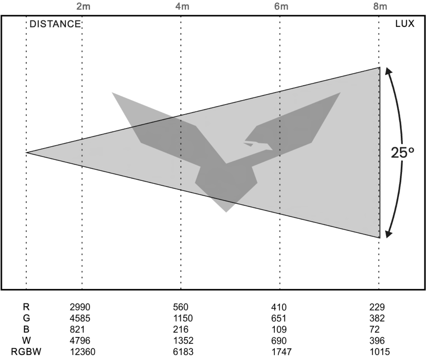
FALCON 270 25° Lens
